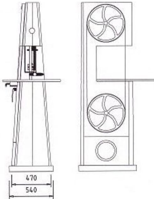
VISTA FRONTAL
